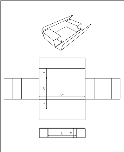
FEFCO 0403
