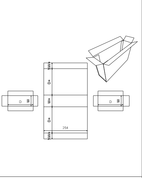
FEFCO 0620
