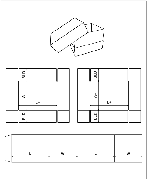
FEFCO 0310
