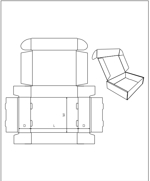
FEFCO 0427
