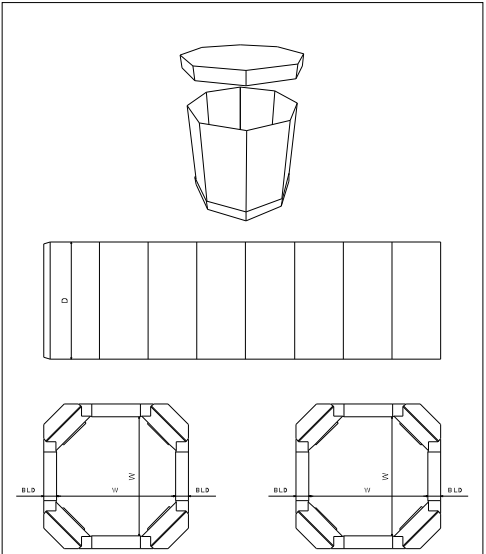
FEFCO 0351
