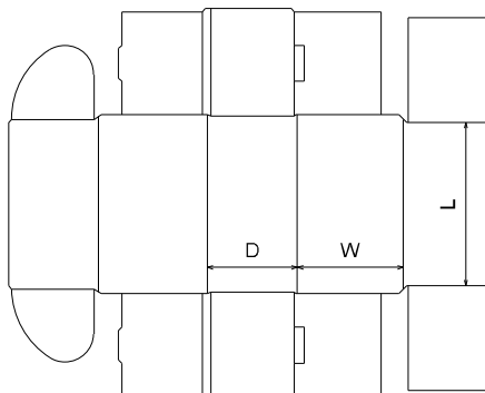
FEFCO 0471
