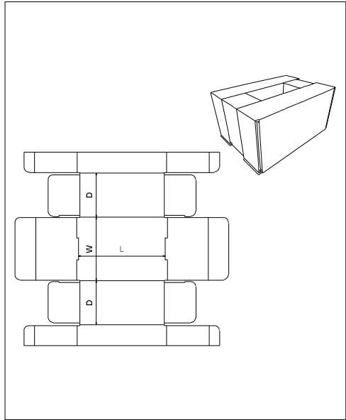
FEFCO 0431
