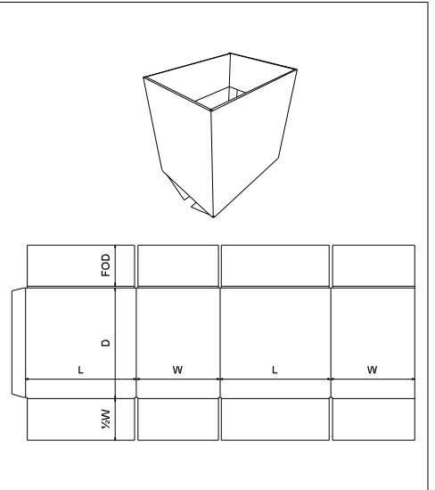
FEFCO 0214
