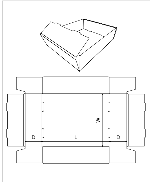
FEFCO 0422
