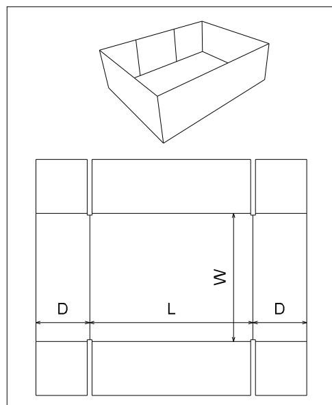
FEFCO 0452
