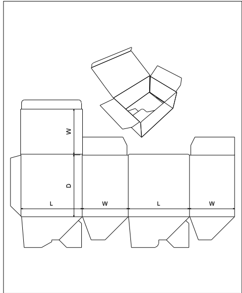
FEFCO 0713
