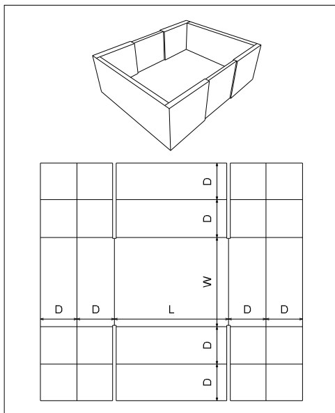
FEFCO 0456
