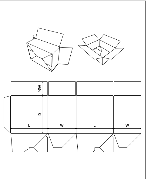
FEFCO 0711
