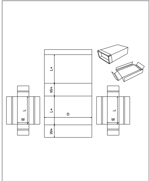
FEFCO 0615
