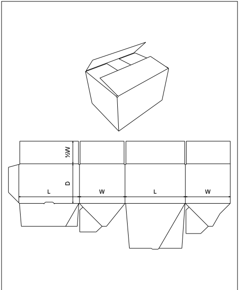
FEFCO 0701
