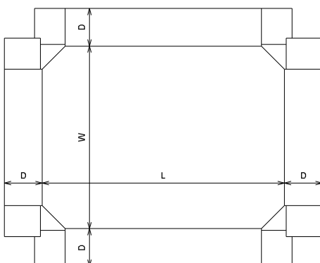
FEFCO 0459
