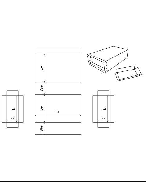
FEFCO 0616
