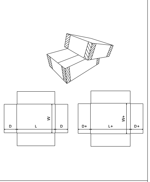
FEFCO 0302
