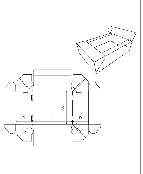
FEFCO 0773
