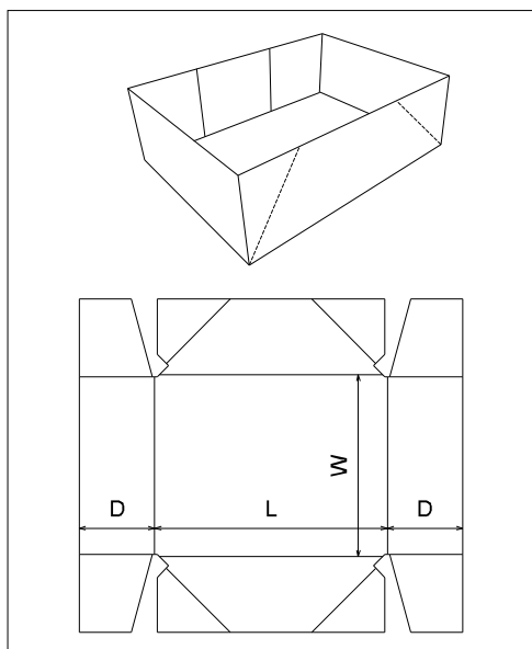
FEFCO 0451
