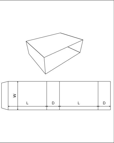
FEFCO 0502
