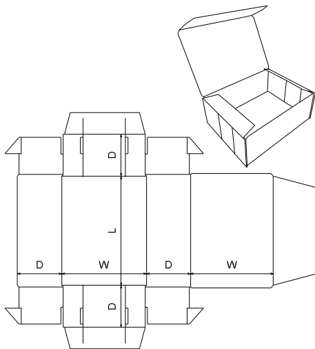
FEFCO 0445
