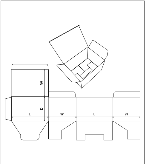
FEFCO 0215
