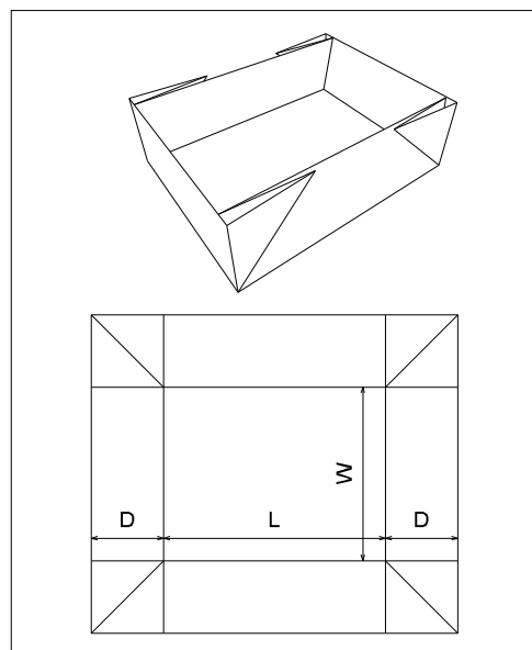
FEFCO 0449
