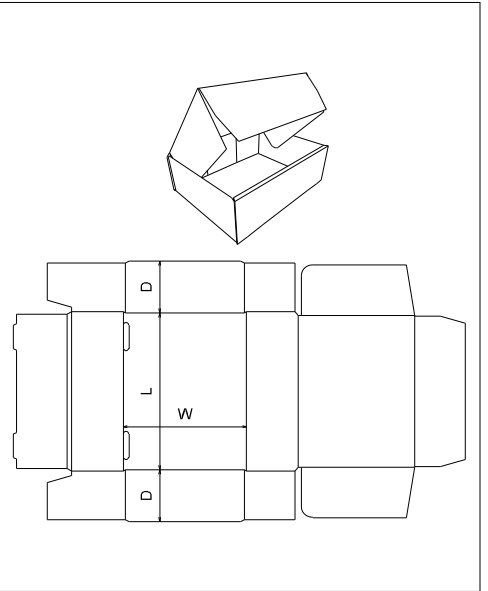
FEFCO 0426
