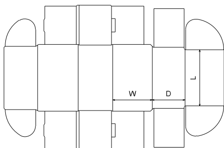
FEFCO 0472
