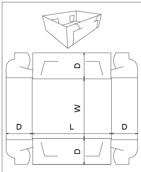
FEFCO 0457
