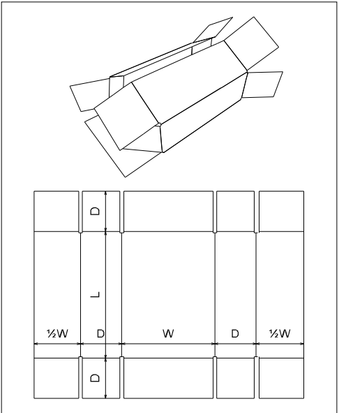
FEFCO 0411
