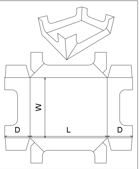
FEFCO 0770
