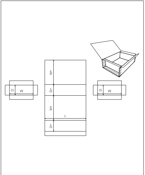
FEFCO 0610
