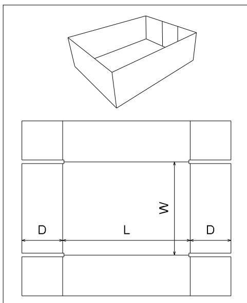
FEFCO 0453
