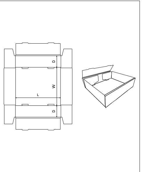
FEFCO 0423
