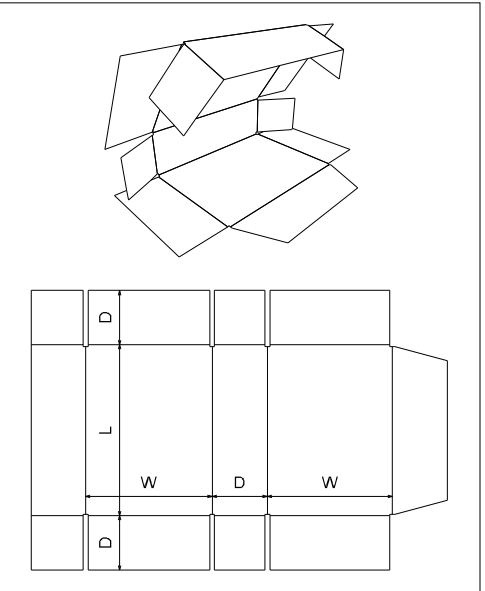
FEFCO 0410
