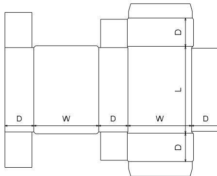
FEFCO 0447
