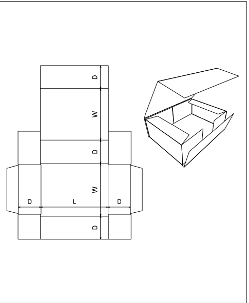
FEFCO 0413
