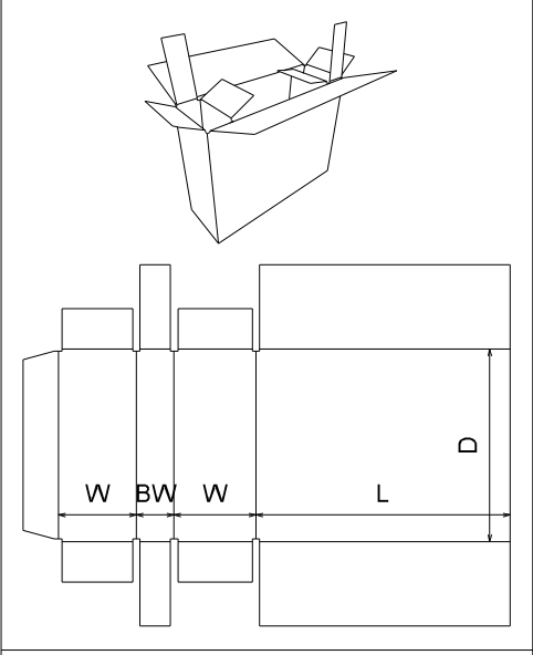
FEFCO 0621
