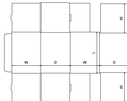
FEFCO 0470
