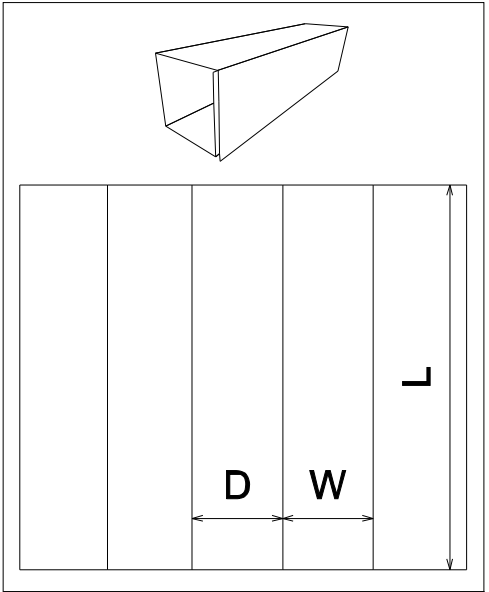
FEFCO 0914
