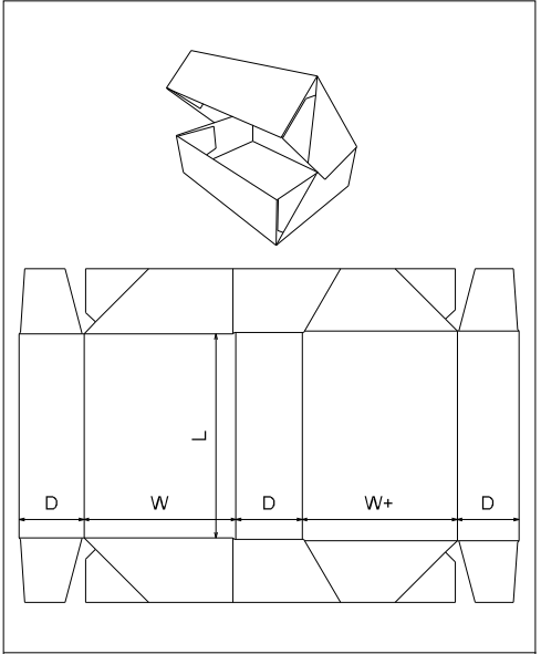
FEFCO 0759
