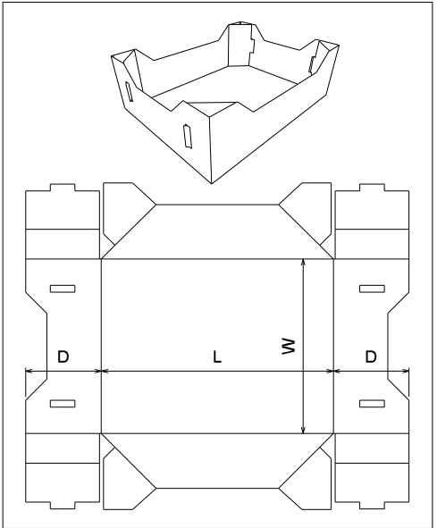
FEFCO 0771
