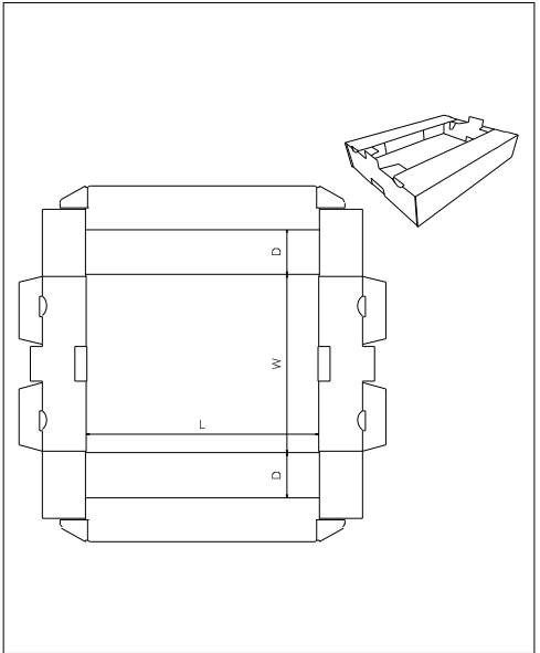
FEFCO 0436
