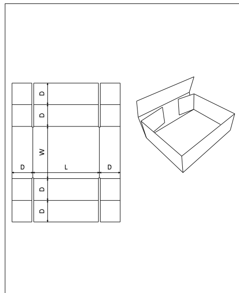
FEFCO 0455
