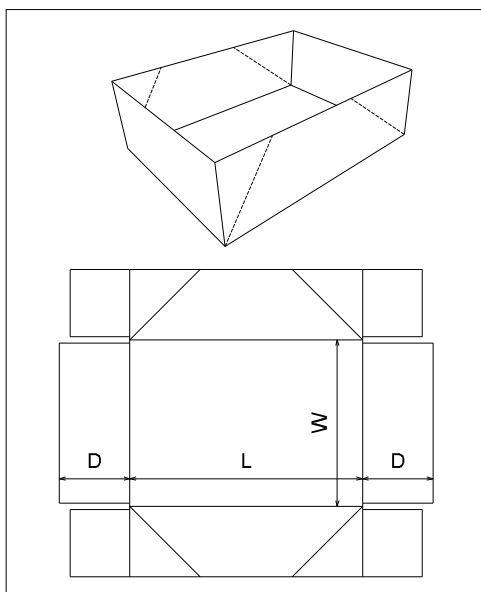
FEFCO 0450
