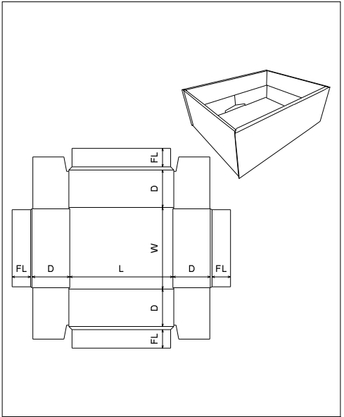
FEFCO 0430
