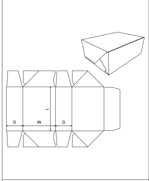
FEFCO 0751
