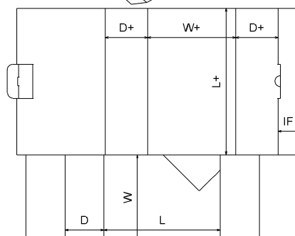
FEFCO 0473
