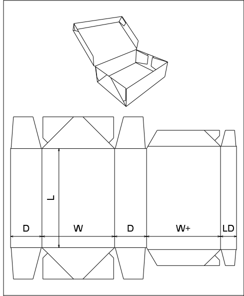
FEFCO 0761
