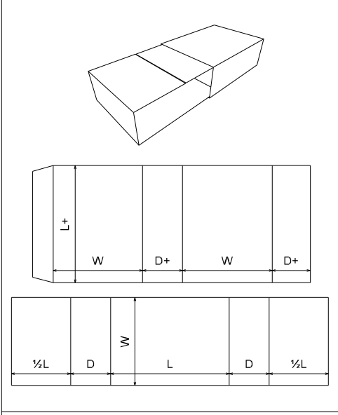
FEFCO 0509
