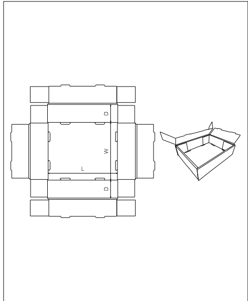
FEFCO 0425
