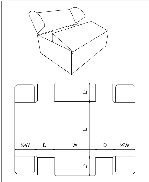
FEFCO 0416
