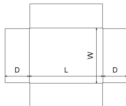
FEFCO 0458
